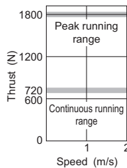
LM-H2P3C-72M-1SS0(*2)
