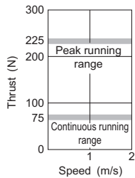
LM-U2P2B-40M-2SSO (*2)
