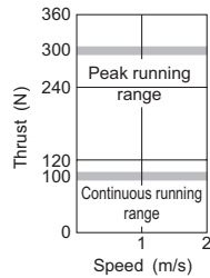
LM-U2PBD-15M-1SSO (*1)
