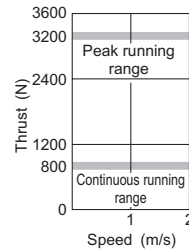
LM-U2P2D-80M-2SSO (*2)
