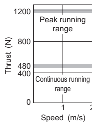
LM-H2P3C-72M-1SS0(*2)
