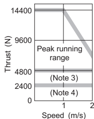
LM-FP4H-48M-1SS0 (*1)
