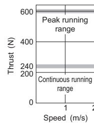
LM-H2P3D-96M-1SS0(*2)
