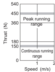
LM-U2P2C-60M-2SSO (*2)
