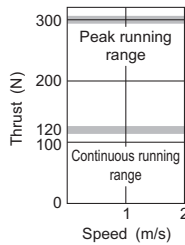
LM-H2P2D-48M-1SS0(*2)
