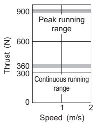
LM-H2P3B-48M-1SS0(*2)
